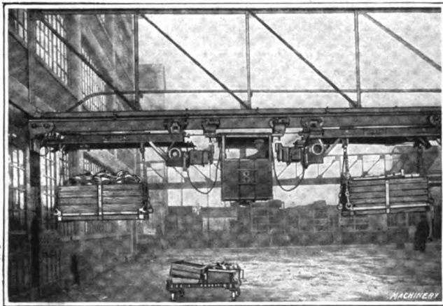
Fig. 1—Where it is desired to transport small pieces on trolleys it is necessary to equip trolleys with a carrier in order that a load approximating the trolley's capacity may be carried at each trip. This view in the Ford Motor Co.'s plant shows trolleys with carriers for handling small castings, built by the Sprague Electric Works, New York City.
